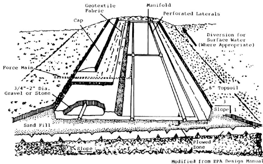
FIGURE 1.2 – DETAILED SCHEMATIC OF A SAND MOUND SYSTEM WITH 3 LATERAL ROWS AND 6 TOTAL LATERALS
